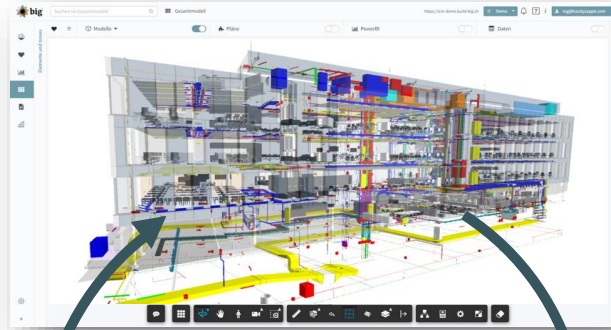
BIM-Modell
